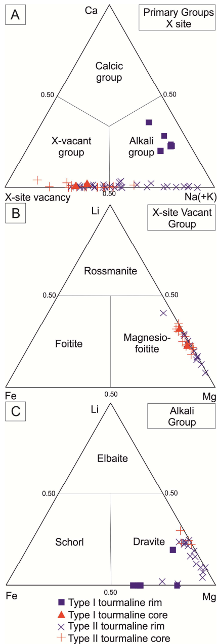
fig 2. Classification of the APV tourmalines by chemical composition in the diagrams proposed by Henry et al. (2011).
