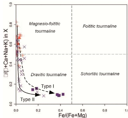
fig 3. Chemical representation of vacancy proportion in X-site versus the Fe/(Fe+Mg) ratio of the APV analysed tourmalines.
