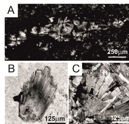
fig 1. Tourmalines from the APV intrusive body under petrographic microscope, transmitted light. A. Vein made up of type I tourmaline radial aggregates. (B, C) Type II tourmaline crystals.
